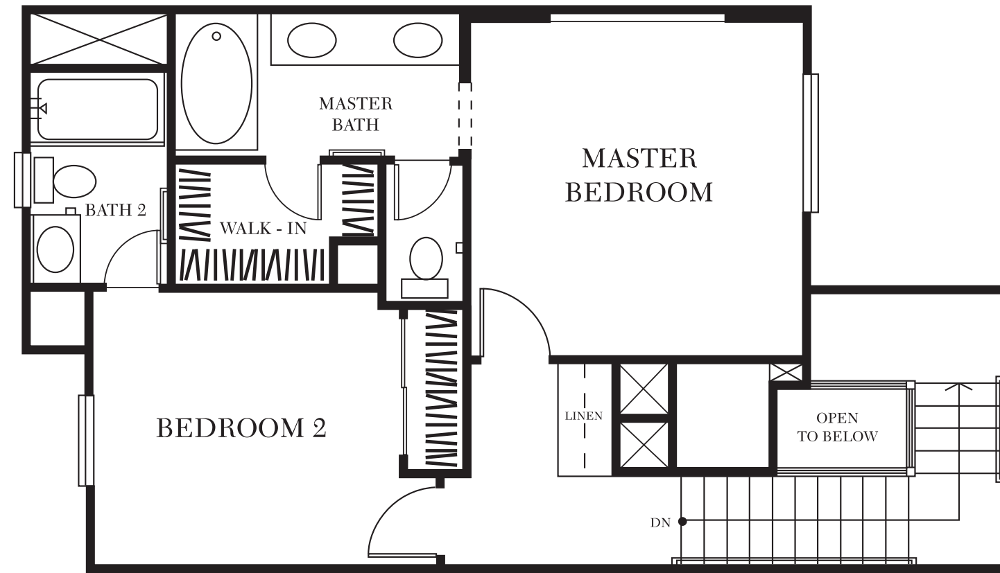
THIRD FLOOR
