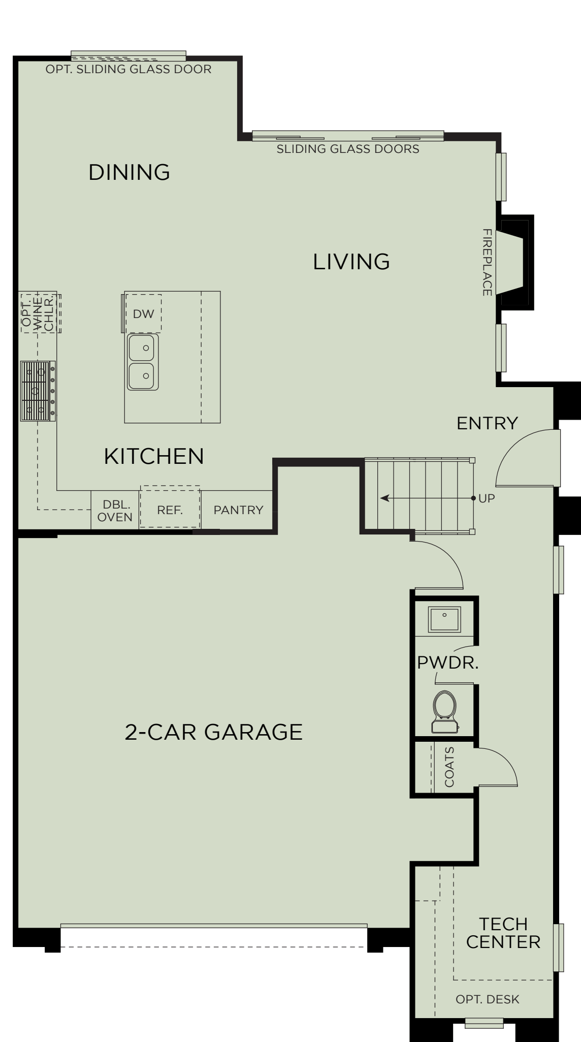
FIRST FLOOR
