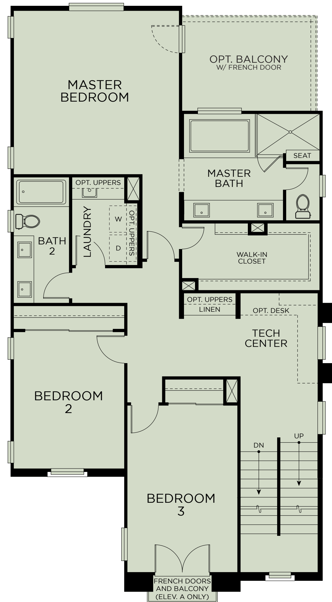
SECOND FLOOR
