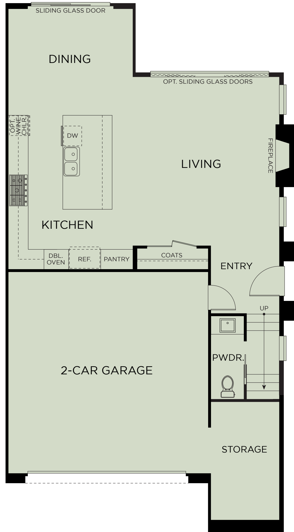
FIRST FLOOR
