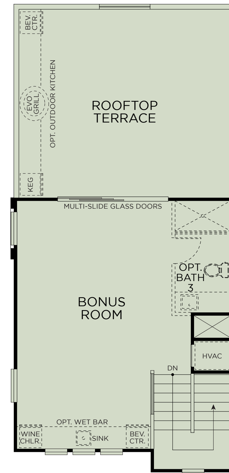
THIRD FLOOR
