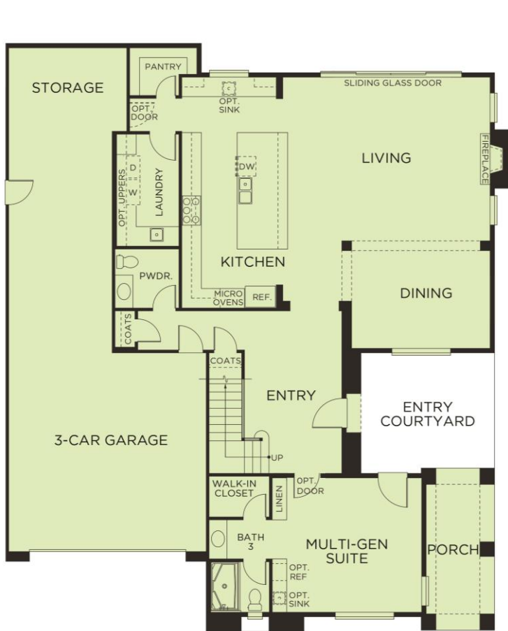
FIRST FLOOR
